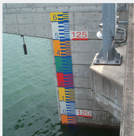
Example: Staff Gauge for Dam
